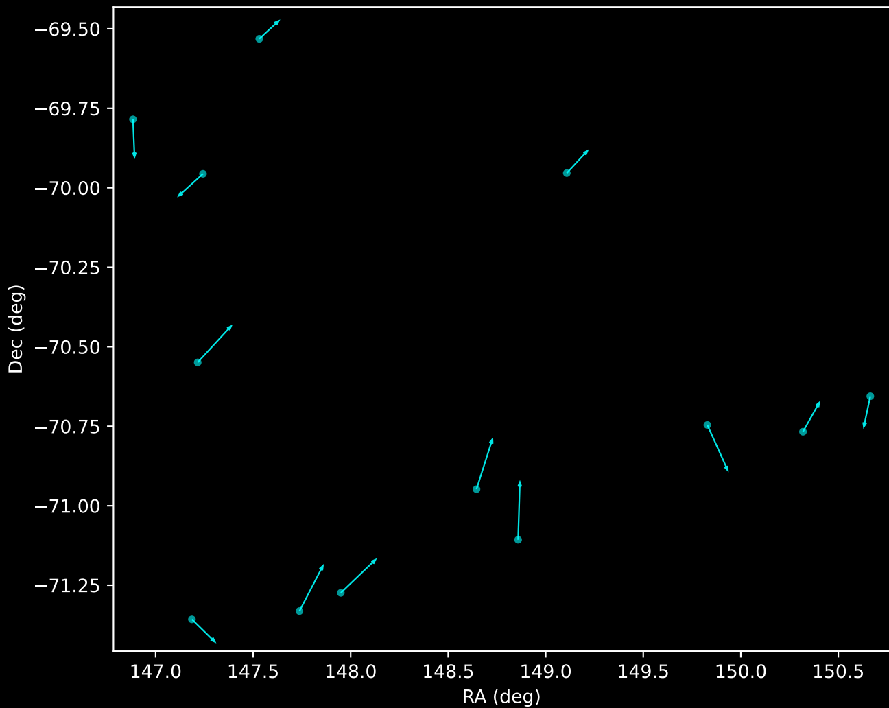
GALAH DR4 Noise Stream Proper Motion Vectors (n=13)
