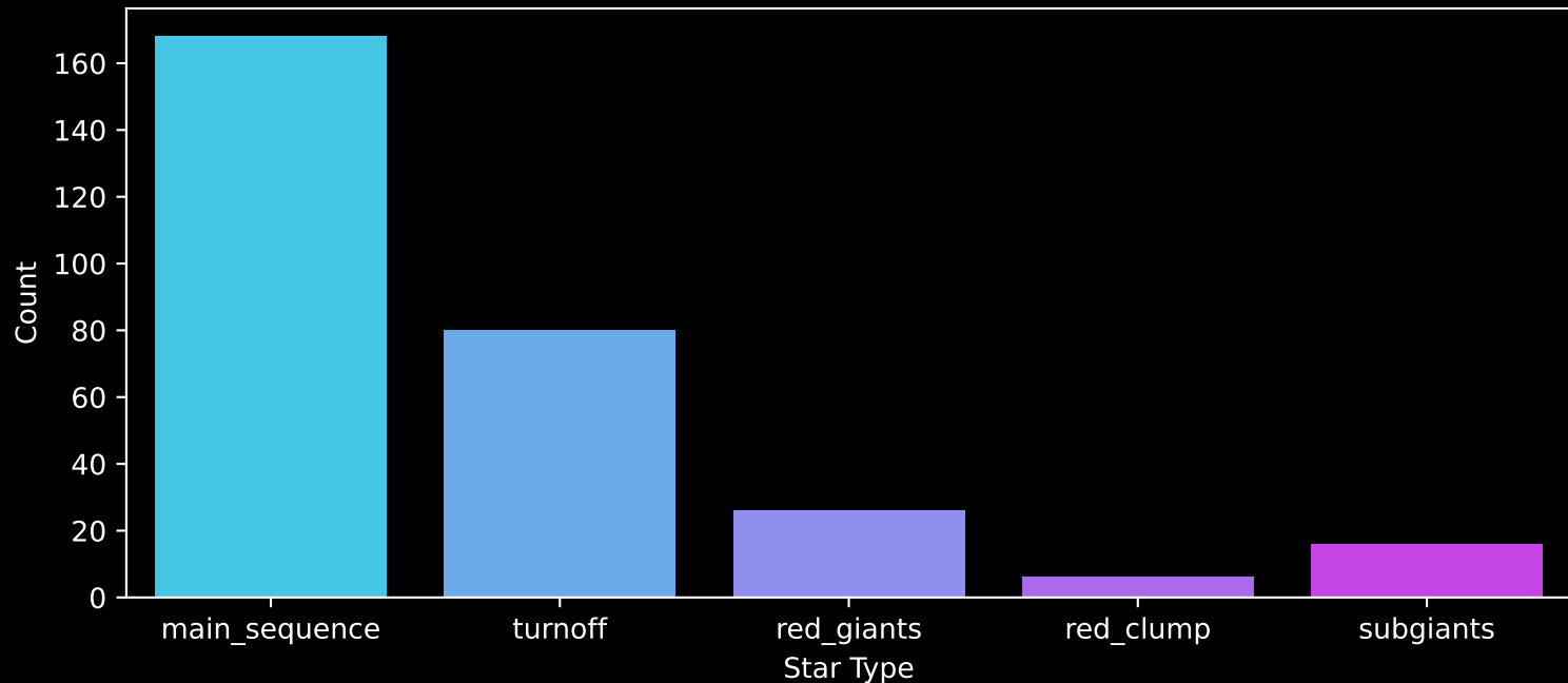
GALAH DR4 Field: [130] Count plot of Star Type
