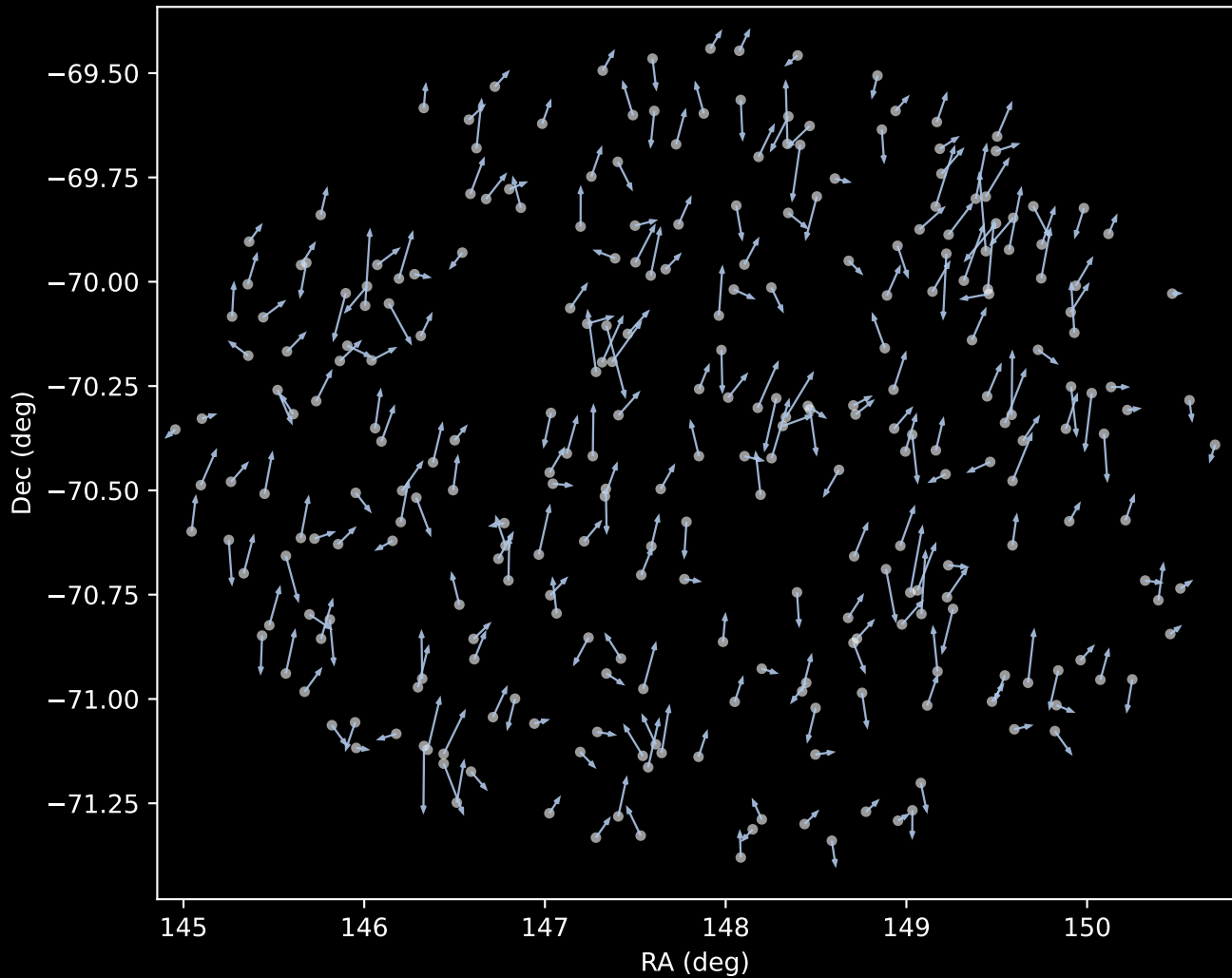
GALAH DR4 Cluster 1 Proper Motion Vectors (n=278)
