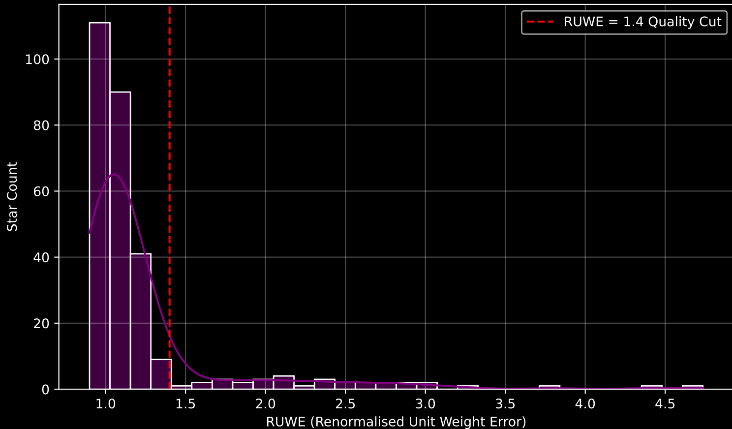
GALAH DR4 Field [130] RUWE Distribution (n= 284)
